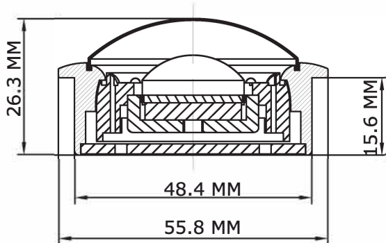
Woofer
