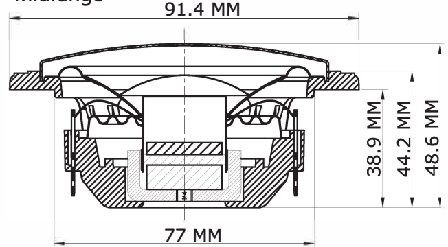
Midrange
