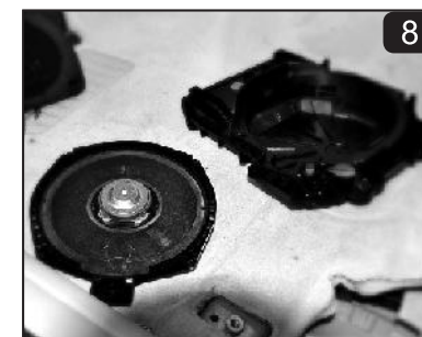
In case of the factory subwoofer is glued, be careful not to damage the plastic enclosure which can be re used for the B2 audio BWF8.
