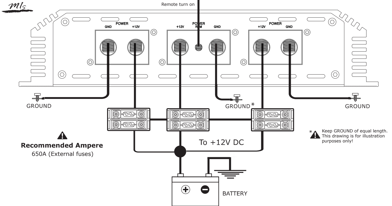
+12V, GND, REM connection chart
